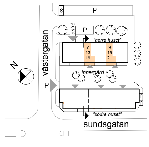
situationsplan
